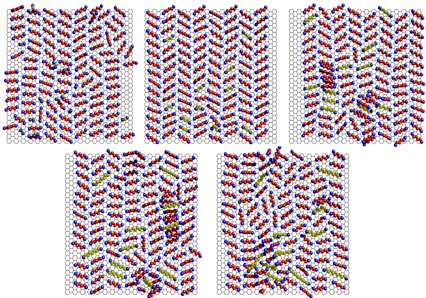
Figure 1. Snapshots of final configurations after 700 ps at T=110\text{K} for 10% propane, pentane, heptane, nonane, and undecane respectively.
